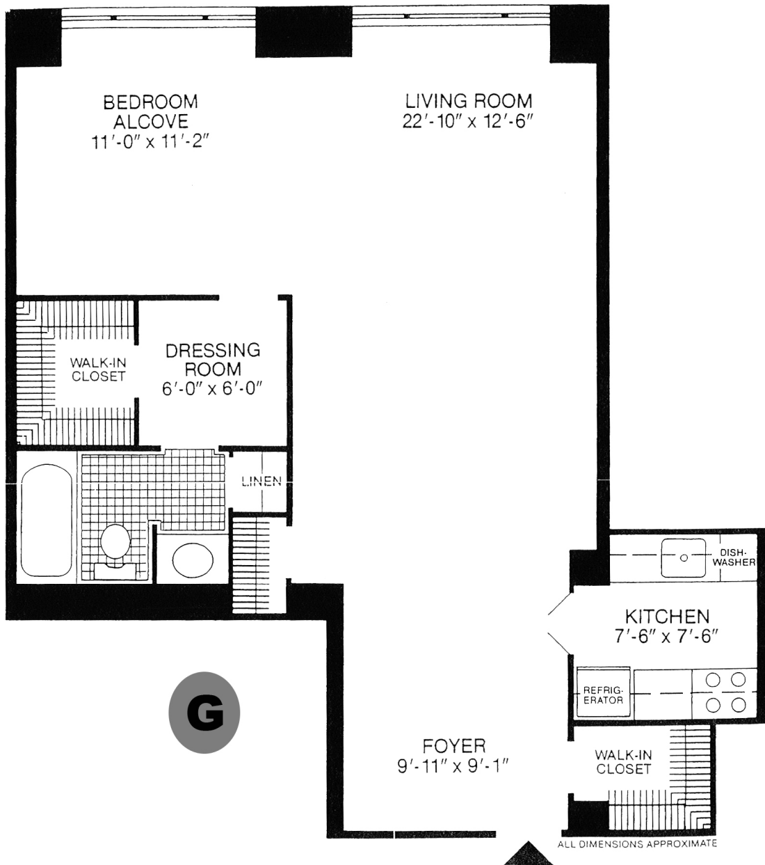
Floor plan for unmodified Unit G
